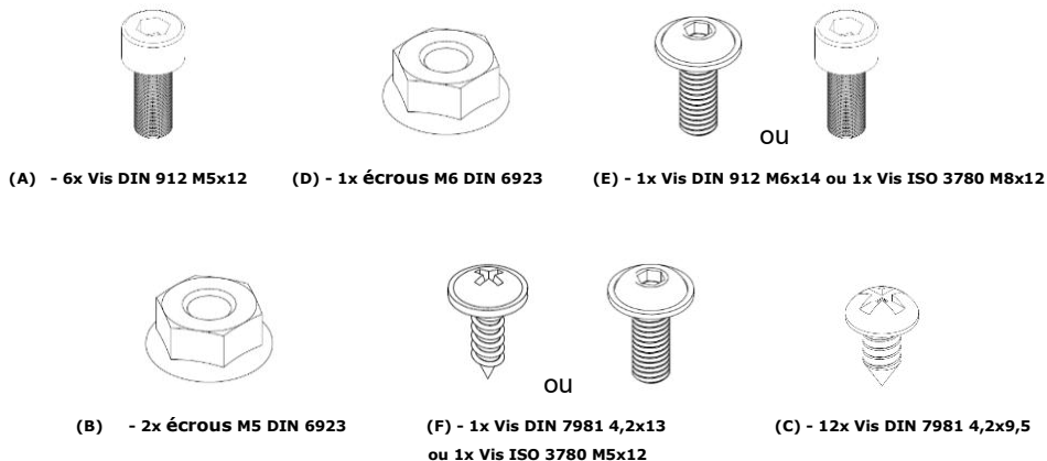
Figure 32 - Kit Olive
