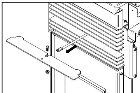
Figure 57 - Montage de la plaque mobile
