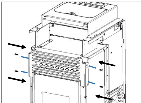
Figure 56 - Fixation grille frontale
