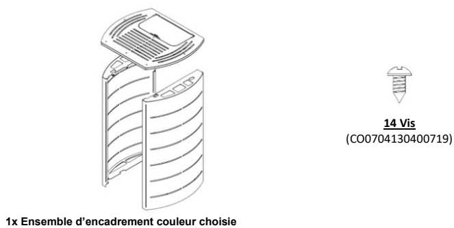
Figure 16 - Kit K2
