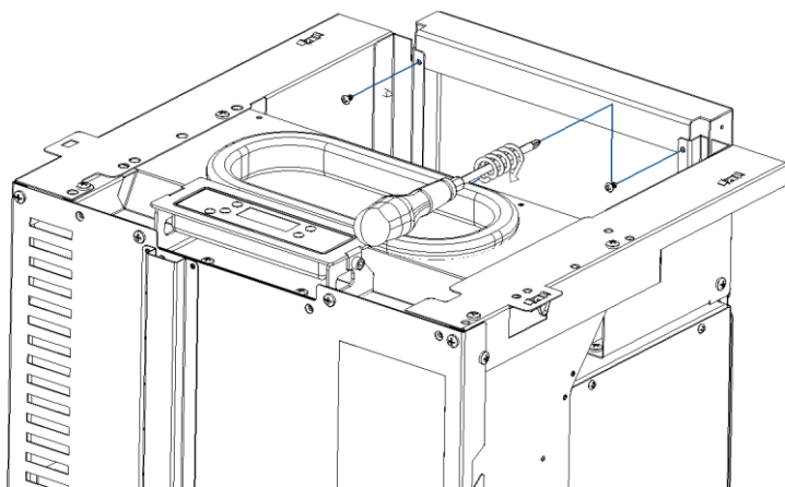
Figure 36 – Fixation de l'habillage frontal
