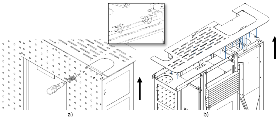
Figure 54 – Retrait couvercle
