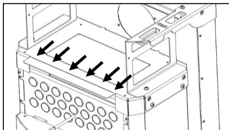
Figure 73 – Retrait visière
