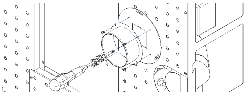
Figure 63 – Fixation buse
