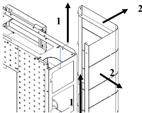
Figure 56 – Retrait habillage
