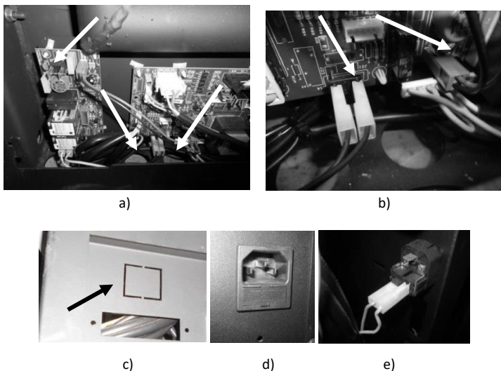
Figure 123 – Installation kit UPS
