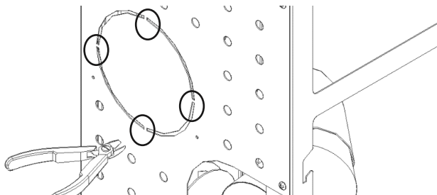
Figure 60 – Retrait tapon
