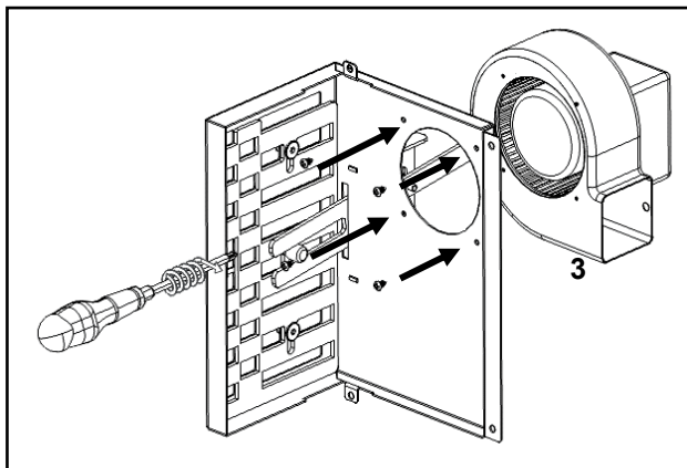
Figure 74 – Fixation support ventilateur
