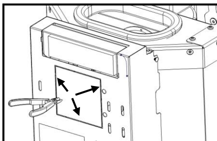
Figure 76 – Retrait couvercle
