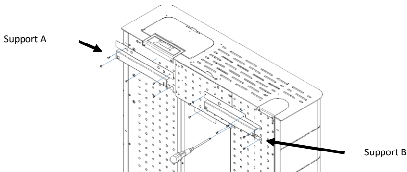
Figure 89 – Montage des supports A et B
