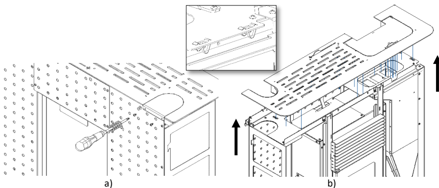
Figure 28 – Retrait couvercle
