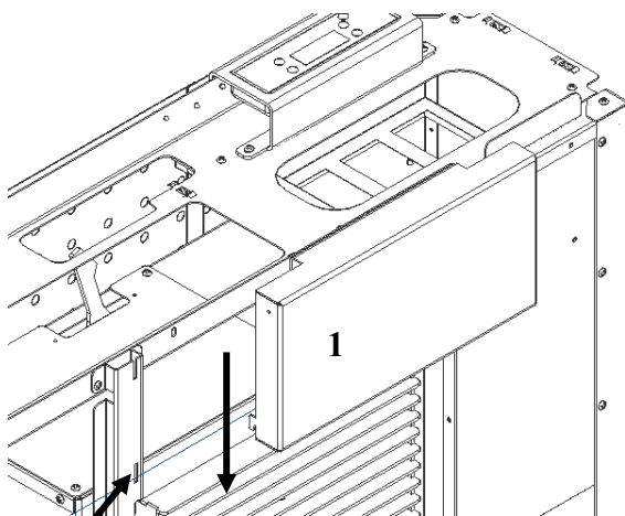
Figure 29 – Placement frontal habillage
