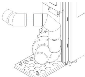
Figure 16 – Raccord coudé en acier inoxydable option 2
